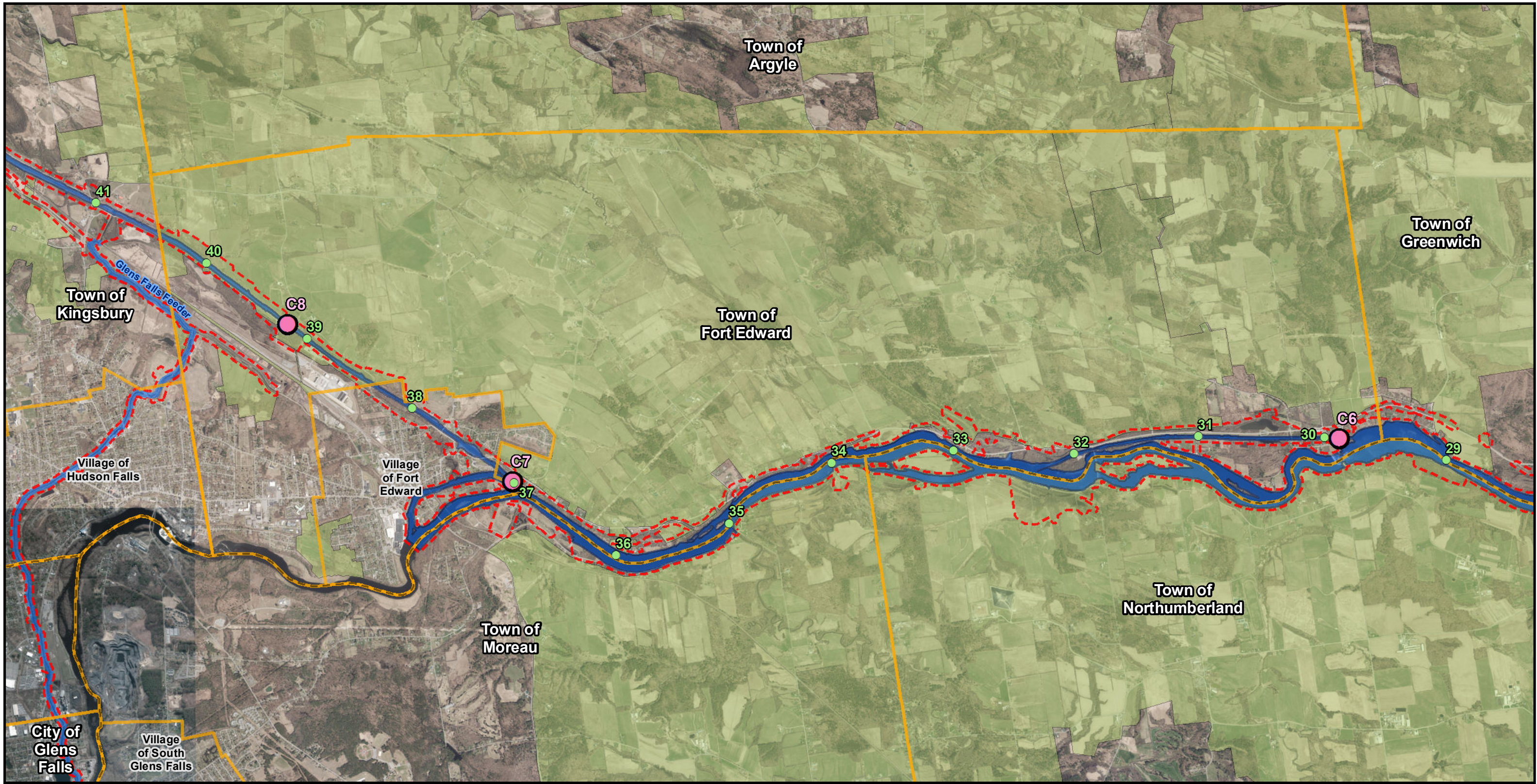
EARTHEN EMBANKMENT INTEGRITY PROGRAM Figure 7E: Units of Special Planning Town and Village of Fort Edward Date: 11/6/2018
